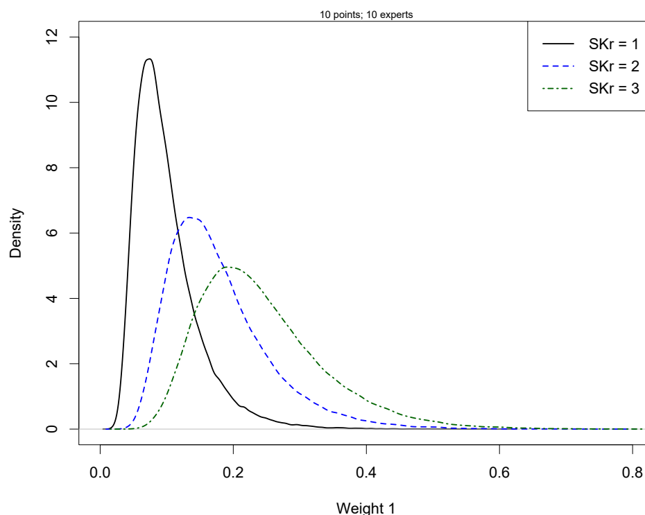
Fig. 7.: Simulated estimated weight distribution for one expert with various skill levels in a 10-expert combination with 10 historical estimation points.
