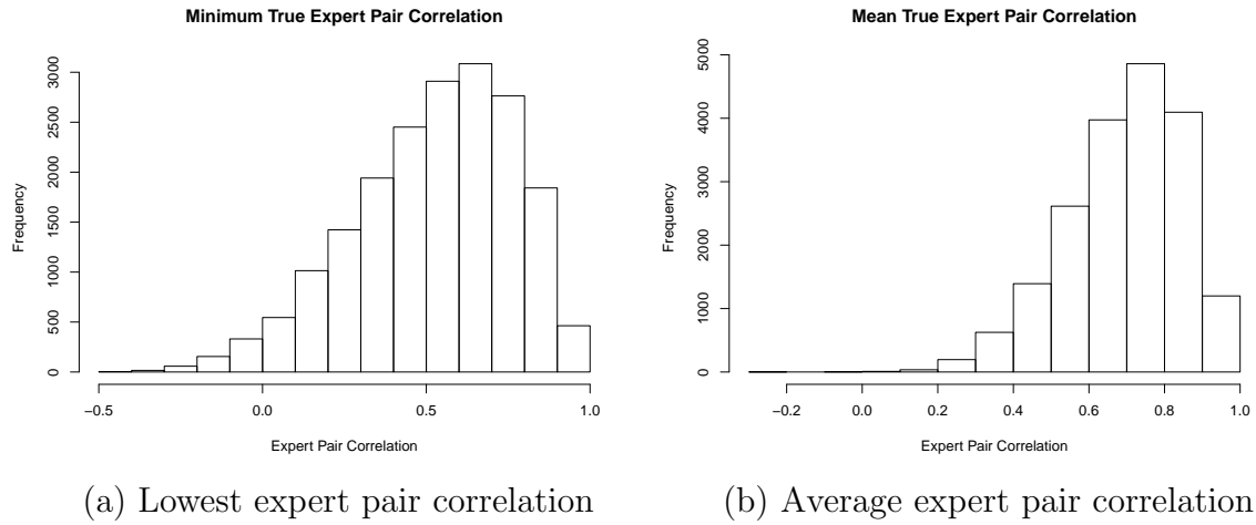
Fig. 24.: Sampling distribution of expert pair correlations used in simulation.
