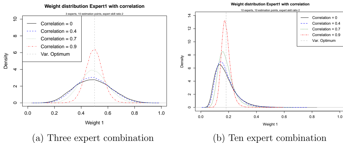
Fig. 19.: Impact of expert correlation levels on estimated weight distribution for variance based weights with 10 historical estimation points based on a simulation. Expert 1 is twice as skillful as all other experts.
